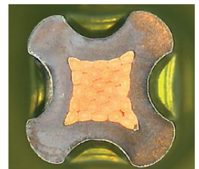
Cross-section of a four-indent crimp
